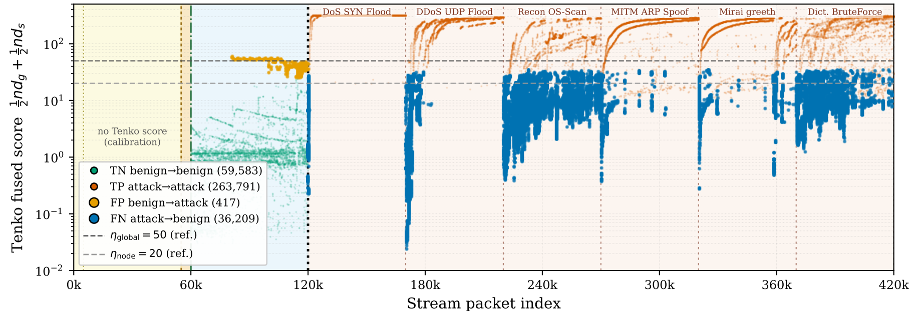
Tenko confusion outcomes (committed \eta = 50/20 ) — CICIoT2023 mixed stream
