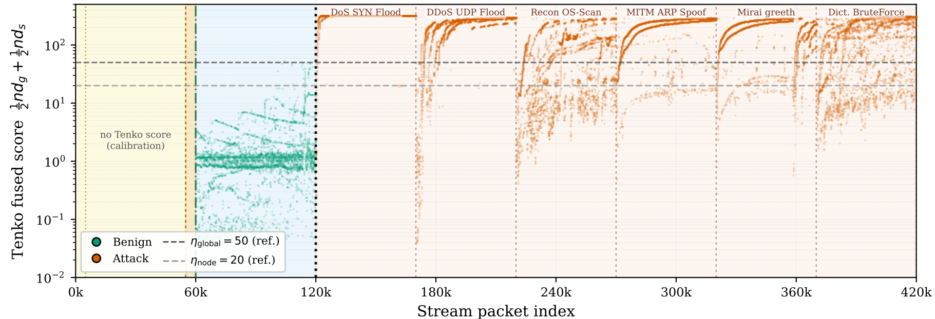
Tenko fused anomaly score (label-colored) — CICIoT2023 mixed stream
