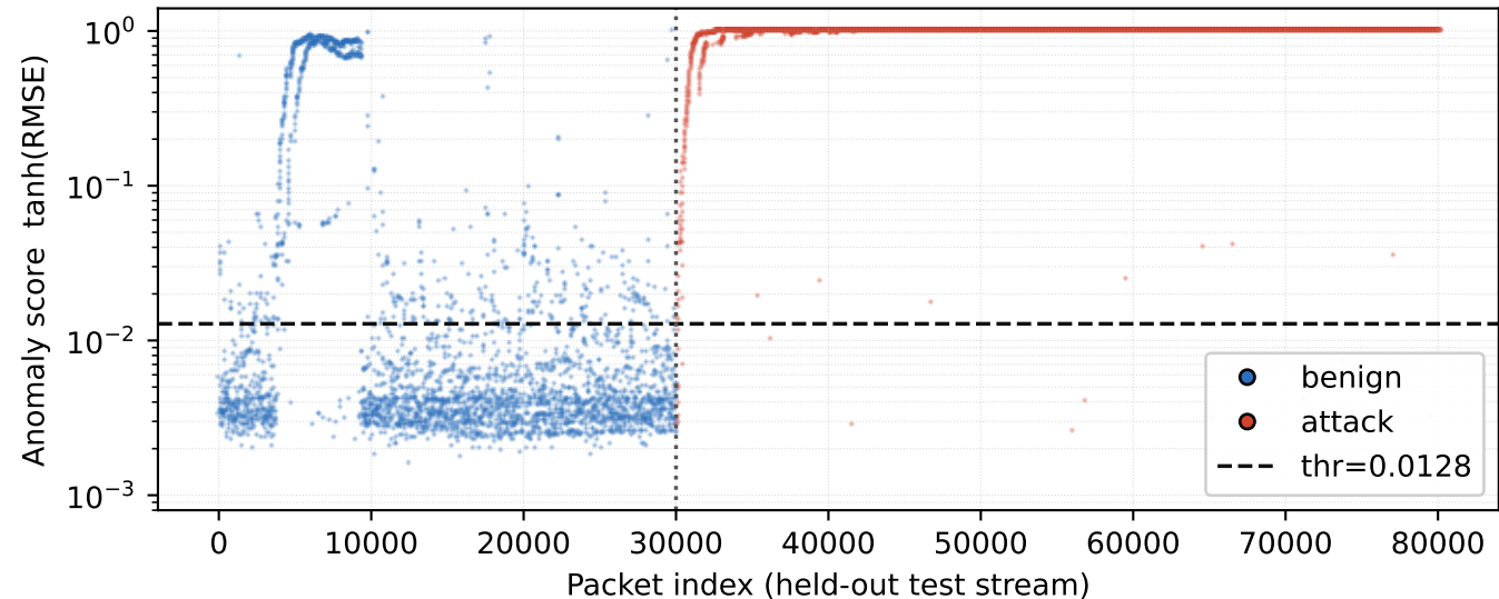
kitsune — DoS-SYN_Flood (from CSV)
