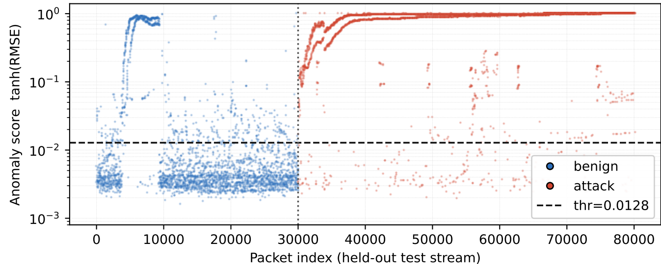
kitsune — MITM-ArpSpoofing (from CSV)
