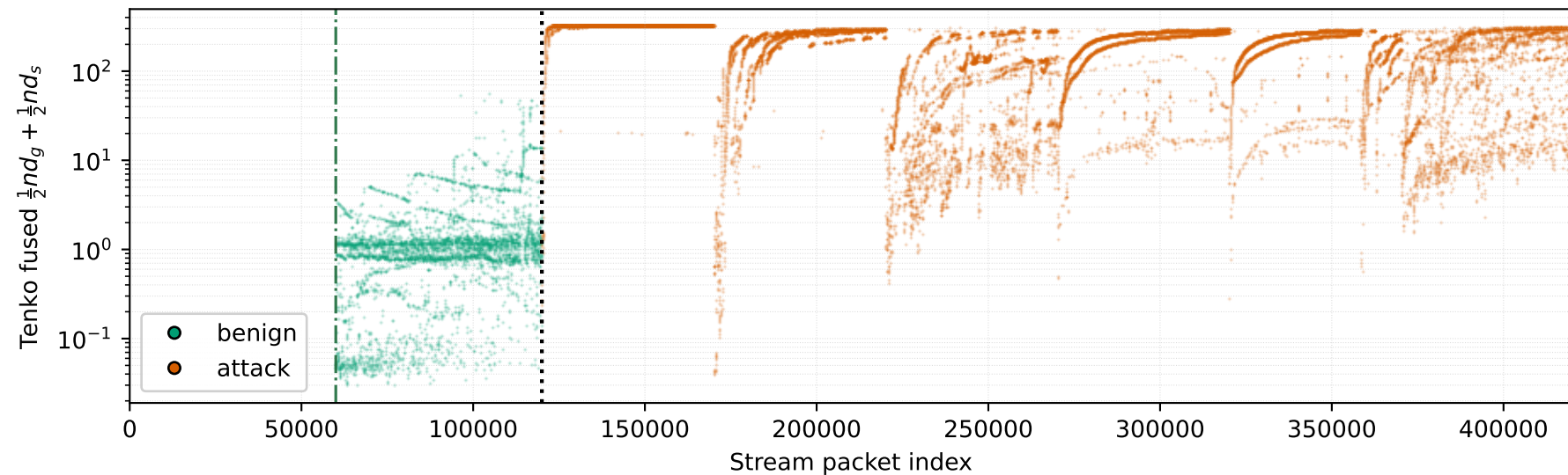
Tenko fused — CICIoT2023 mixed (from CSV)
