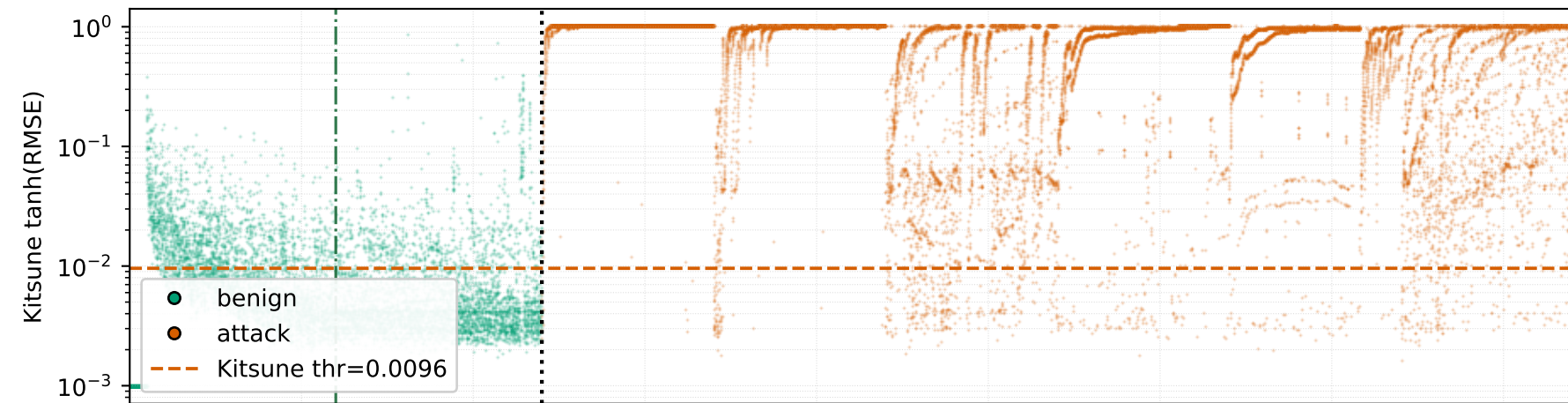
Kitsune — CICIoT2023 mixed (from CSV)
