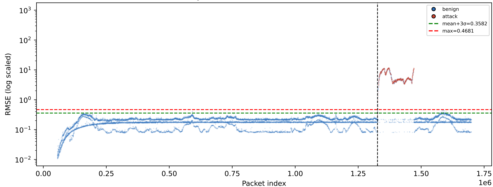
Anomaly Scores — Kitsune OS Scan (from CSV)
