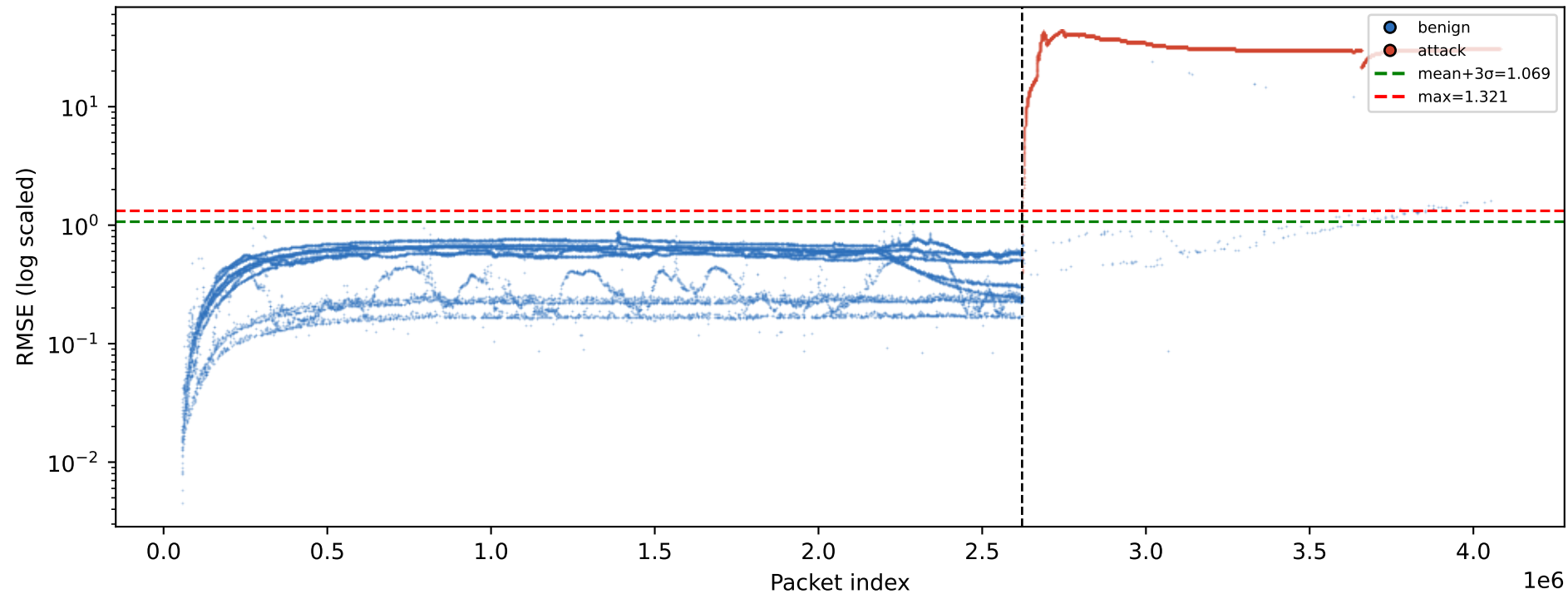
Anomaly Scores — Kitsune SSDP Flood (from CSV)
