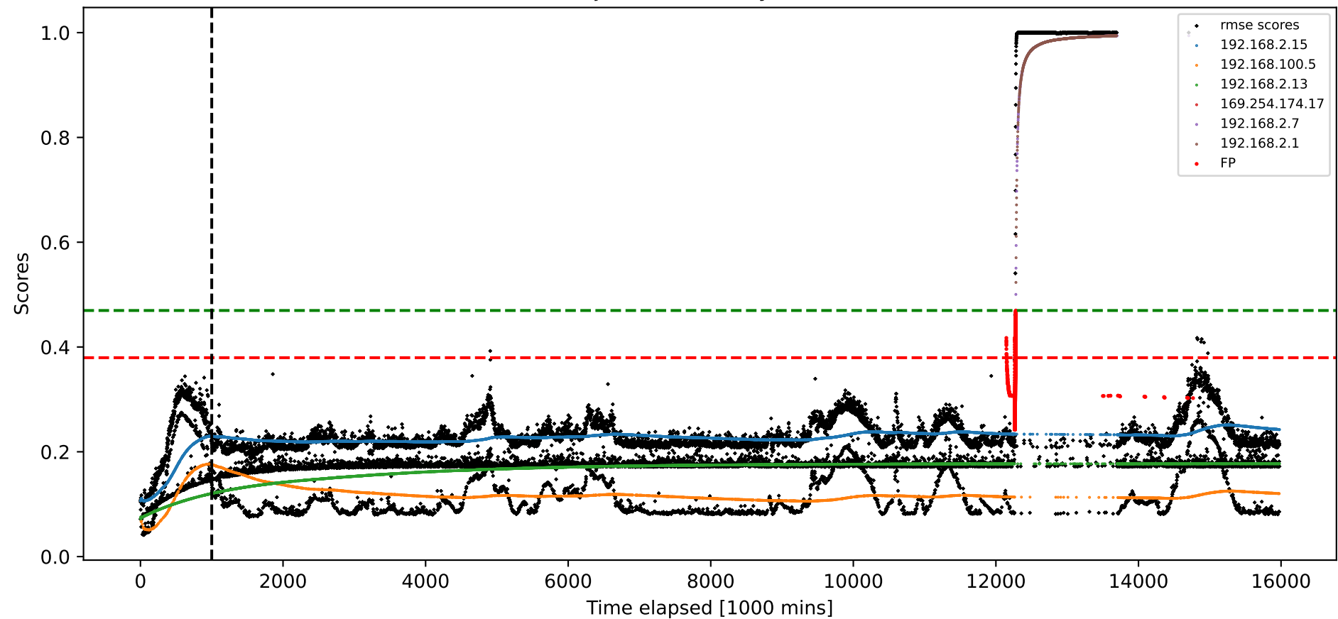
Adjusted Anomaly Scores
