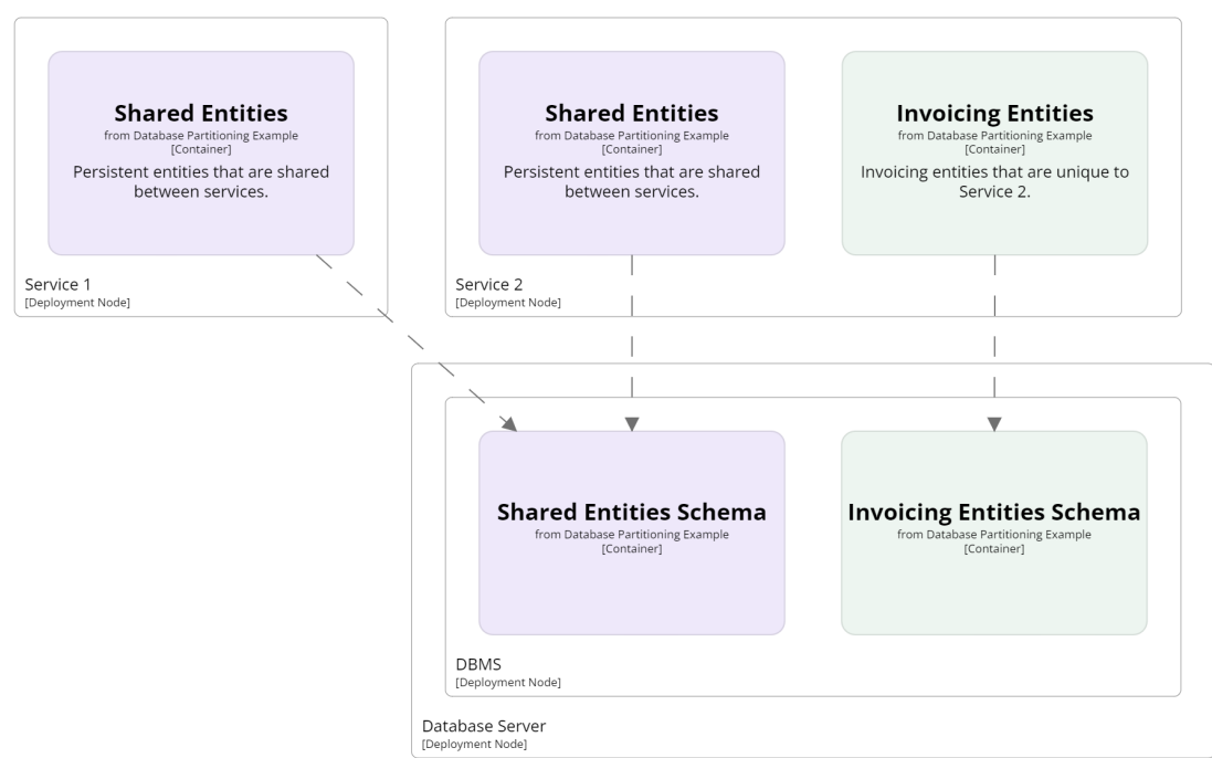
Figure 3: Database logical partitioning example.
