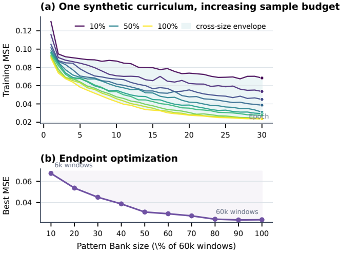
Fig. 7. Pattern Bank optimization from 10% to 100%. (a) Training trajectories and their cross-size envelope. (b) Best training MSE against the nested number of generated windows. Every size uses the same generator mixture and seed.
