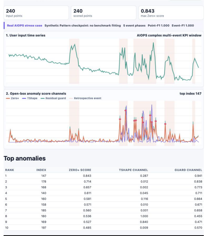
Fig. 15. Released web scorer on a complex real 240-point AIOPS incident window. The interface returns the aligned KPI trace, fused/neural/guard scores, and ranked suspicious points from the same scorer used by the CLI.
