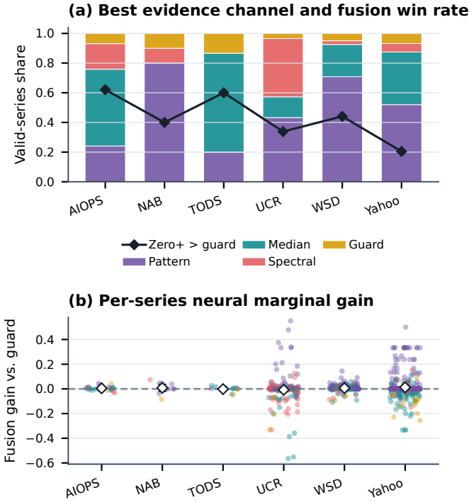
Fig. 12. EasyTSAD channel attribution over paired valid series. (a) Stacked bars identify the strongest individual evidence channel; diamonds show how often final fusion beats the exactly matched guard. (b) Each jittered point is one KPI’s final-fusion gain over that guard, colored by its strongest individual channel; diamonds and whiskers report the dataset mean and 95% bootstrap CI.
