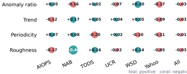
(b) KPI trait vs. neural marginal gain (Spearman \rho )
