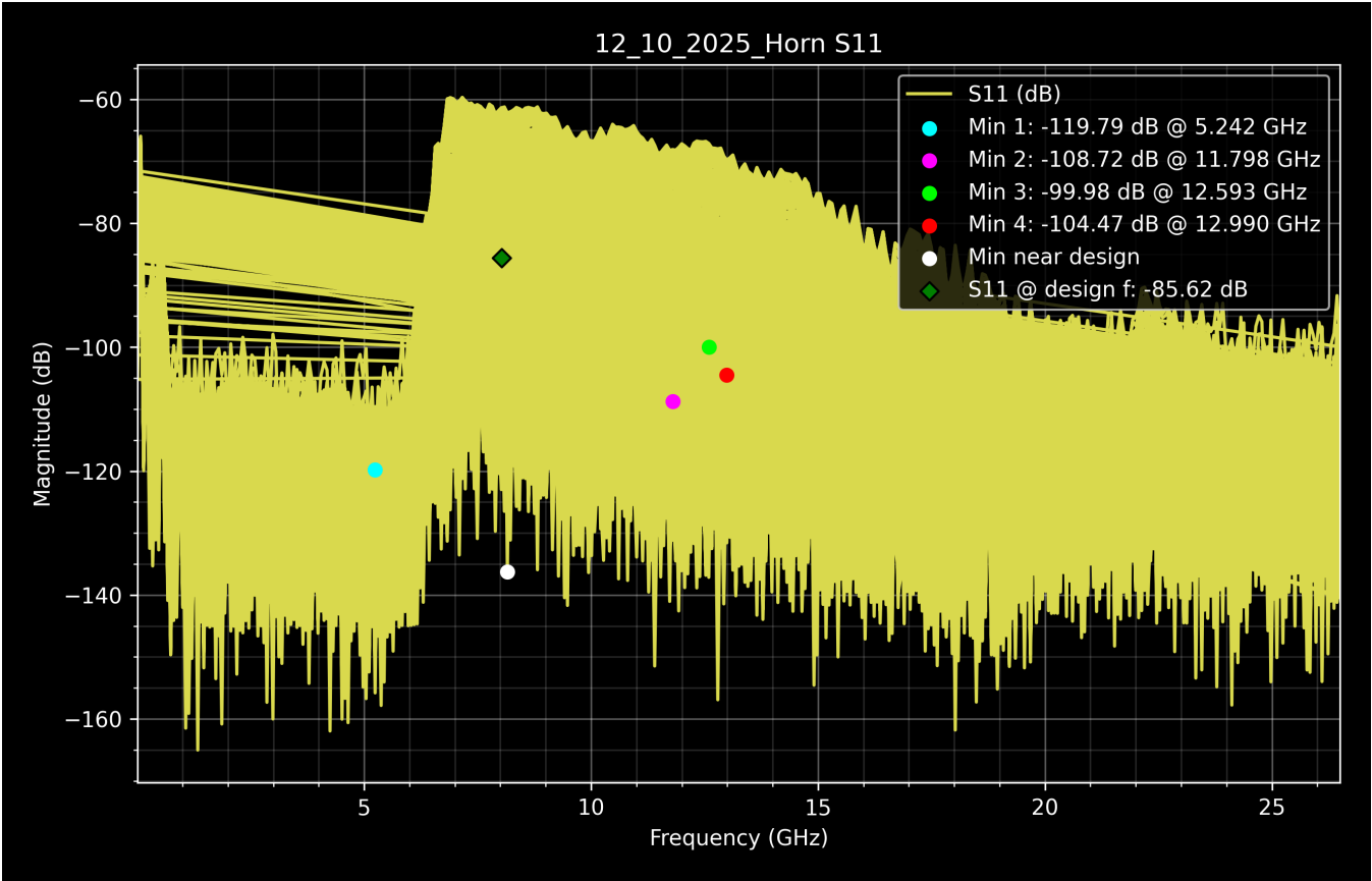
S11 Plot
