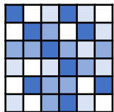
scRNA-seq count matrix
