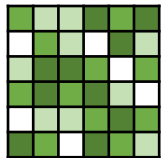
scATAC-seq count matrix
