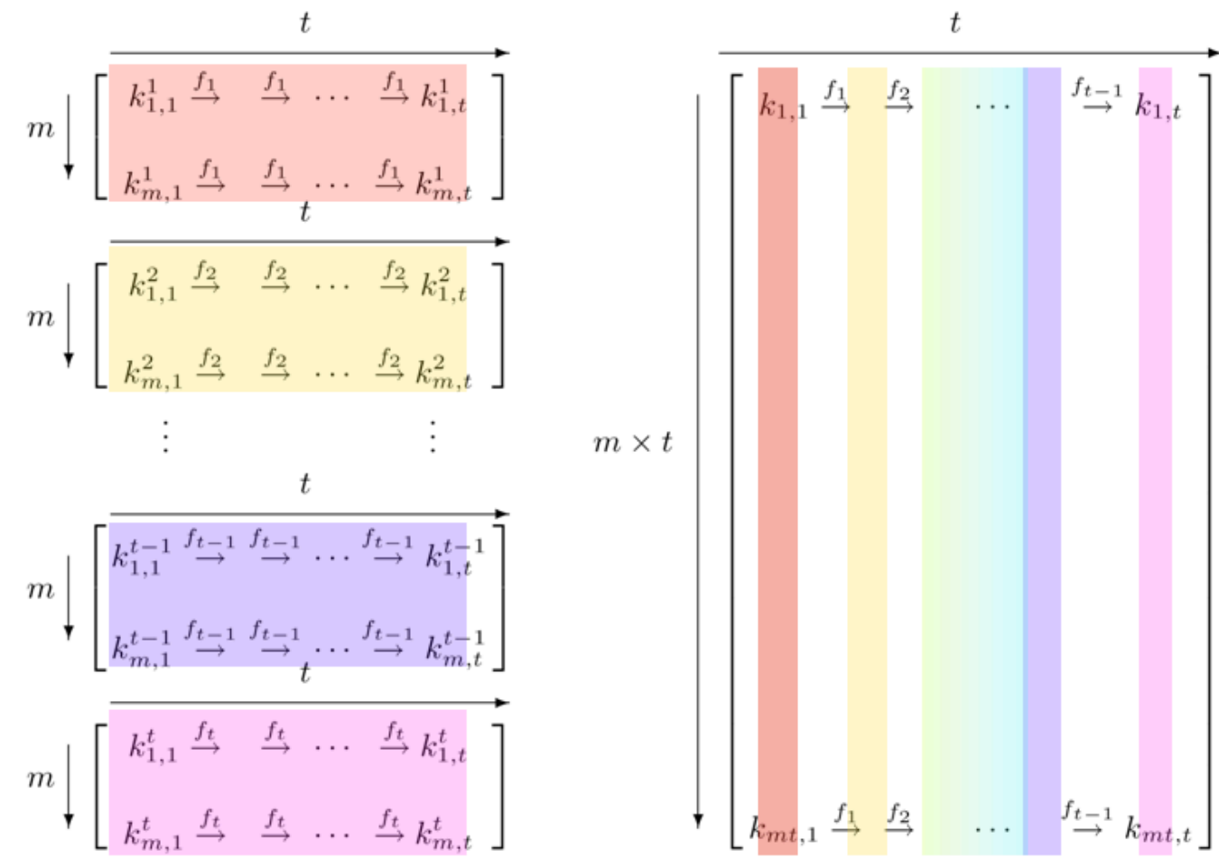
Rainbow Table illustration presented at Crypto 2003
