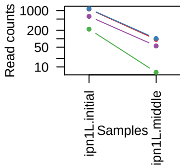
sgRNAs in FBL
