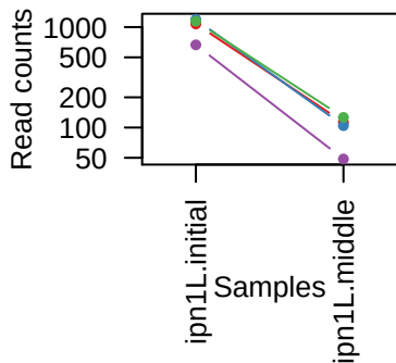
sgRNAs in NOP58
