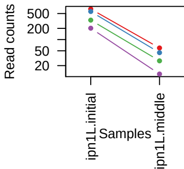
sgRNAs in EIF6
