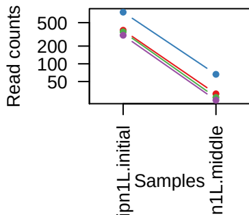
sgRNAs in NOP58
