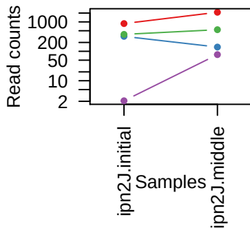
sgRNAs in MS4A6A
