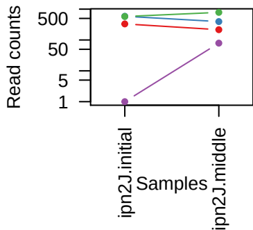
sgRNAs in ZNF713
