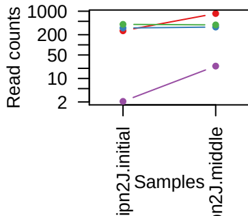
sgRNAs in MS4A6A
