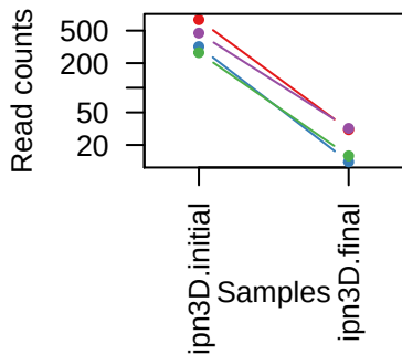
sgRNAs in RAD51C
