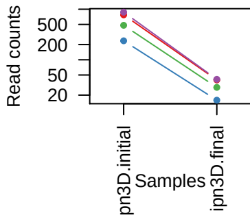
sgRNAs in RAD51C
