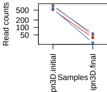
sgRNAs in RPS18
