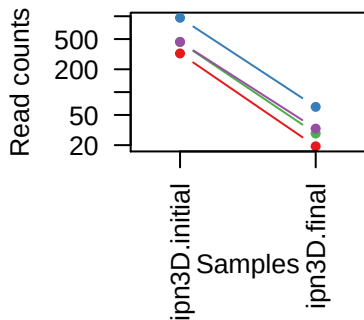
sgRNAs in RPS18
