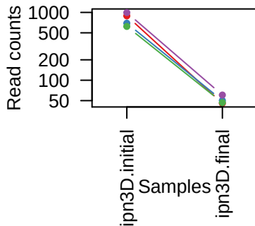
sgRNAs in RRM1
