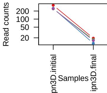
sgRNAs in RRM1
