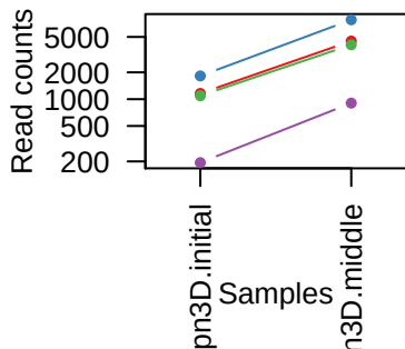
sgRNAs in KCTD5
