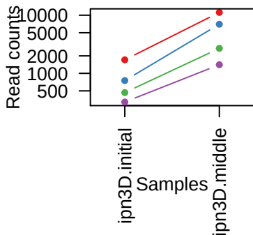
sgRNAs in ARNT
