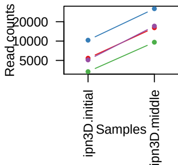
sgRNAs in KCTD5
