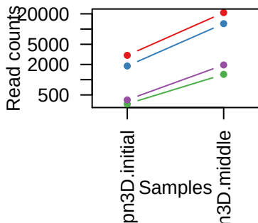
sgRNAs in ARNT
