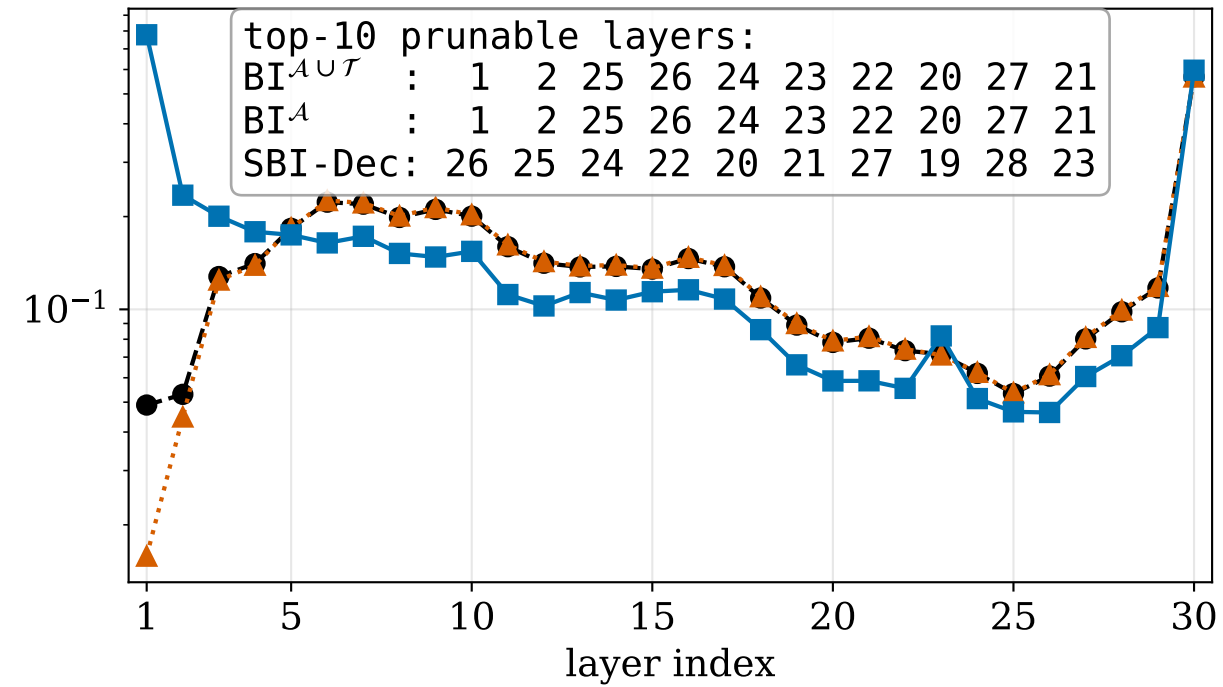
Voxtral
