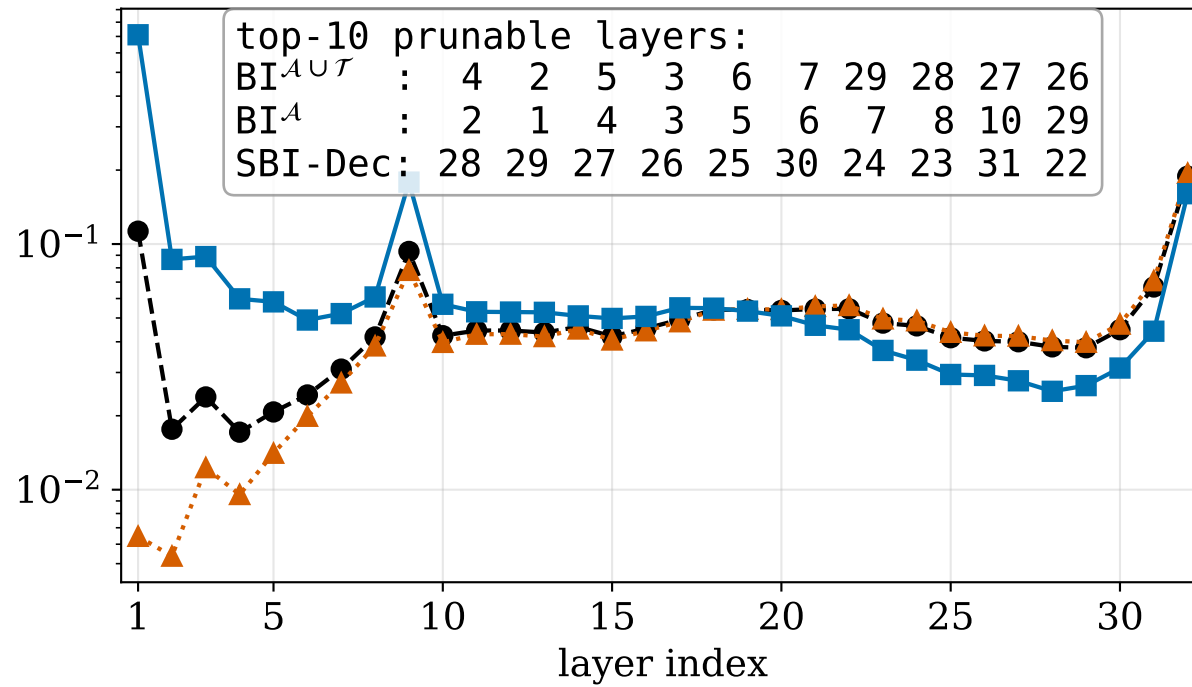
Qwen2-Audio
