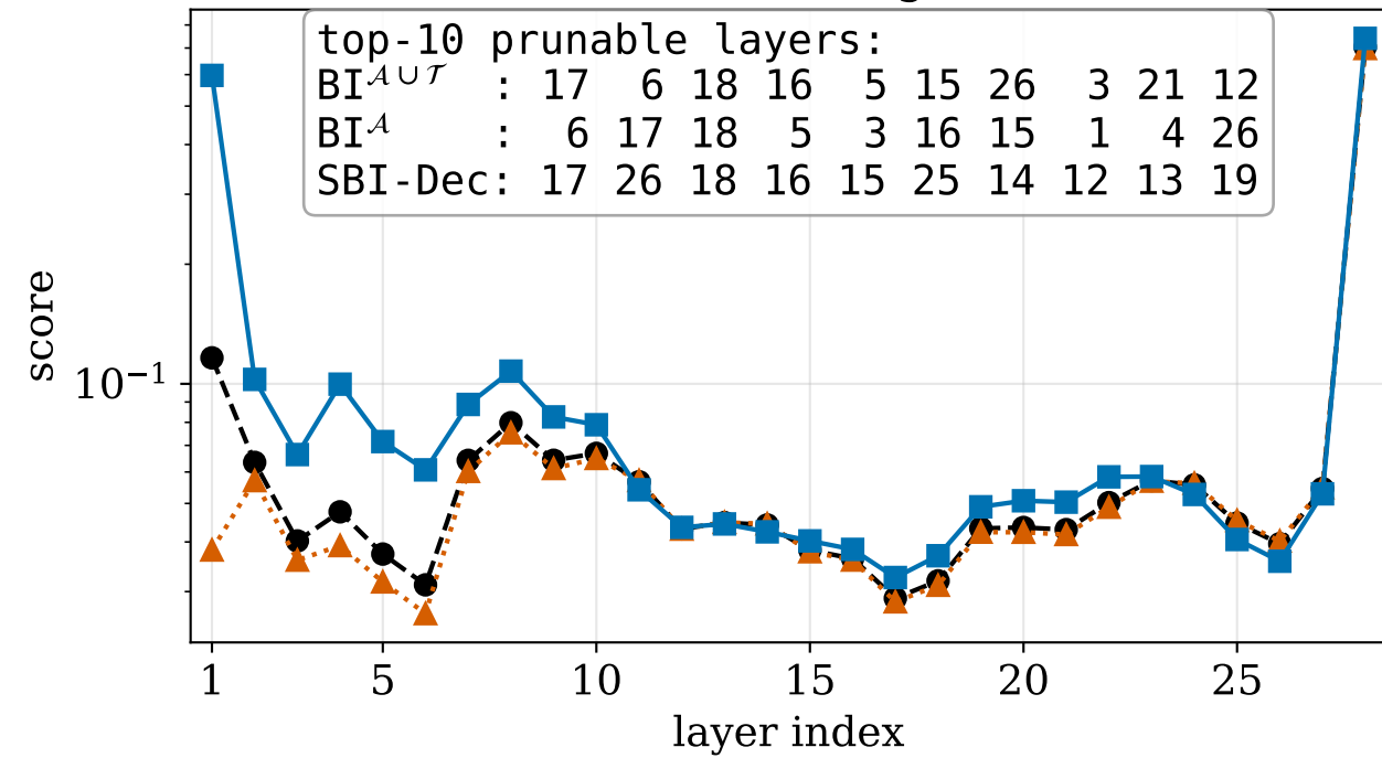
Audio Flamingo 3
