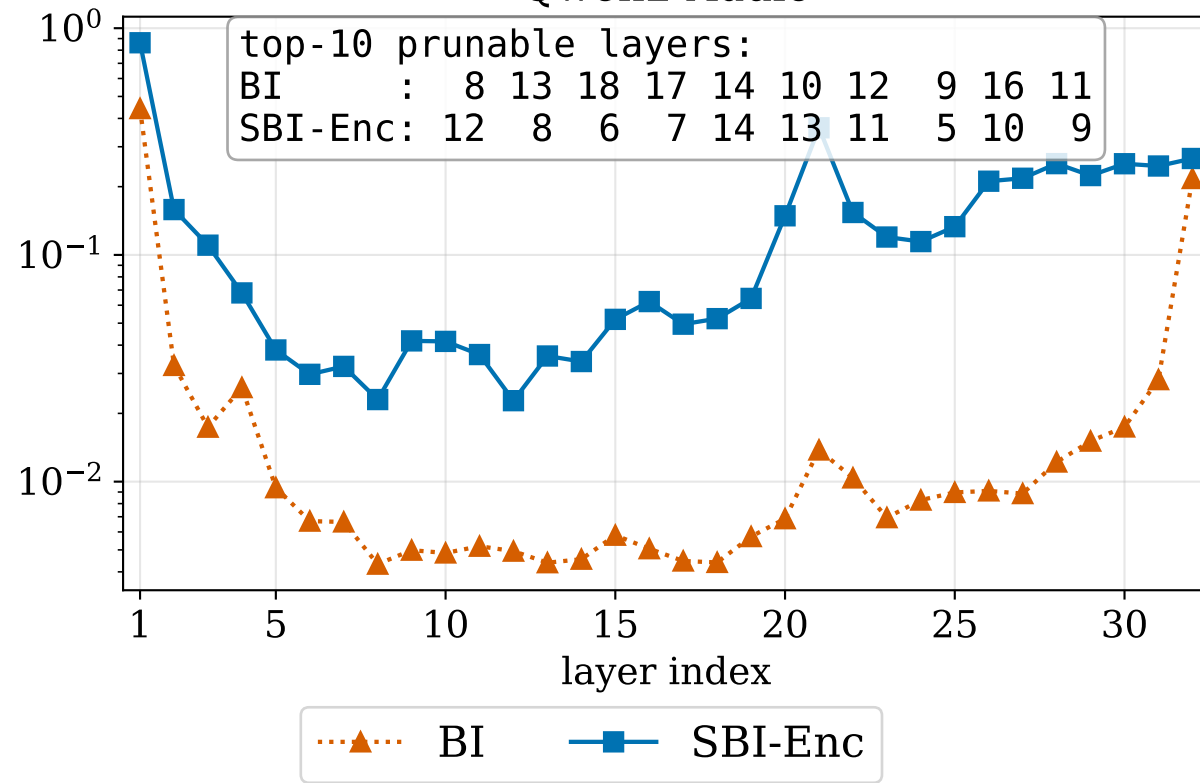
Qwen2-Audio
