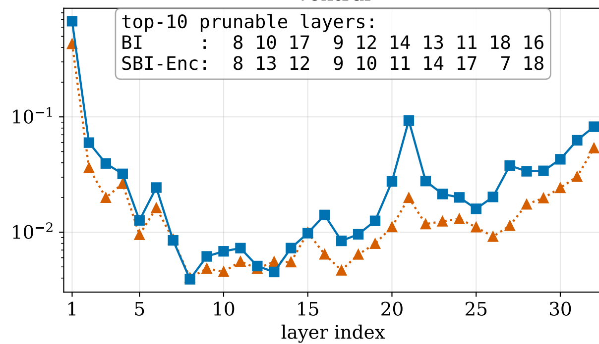
Voxtral
