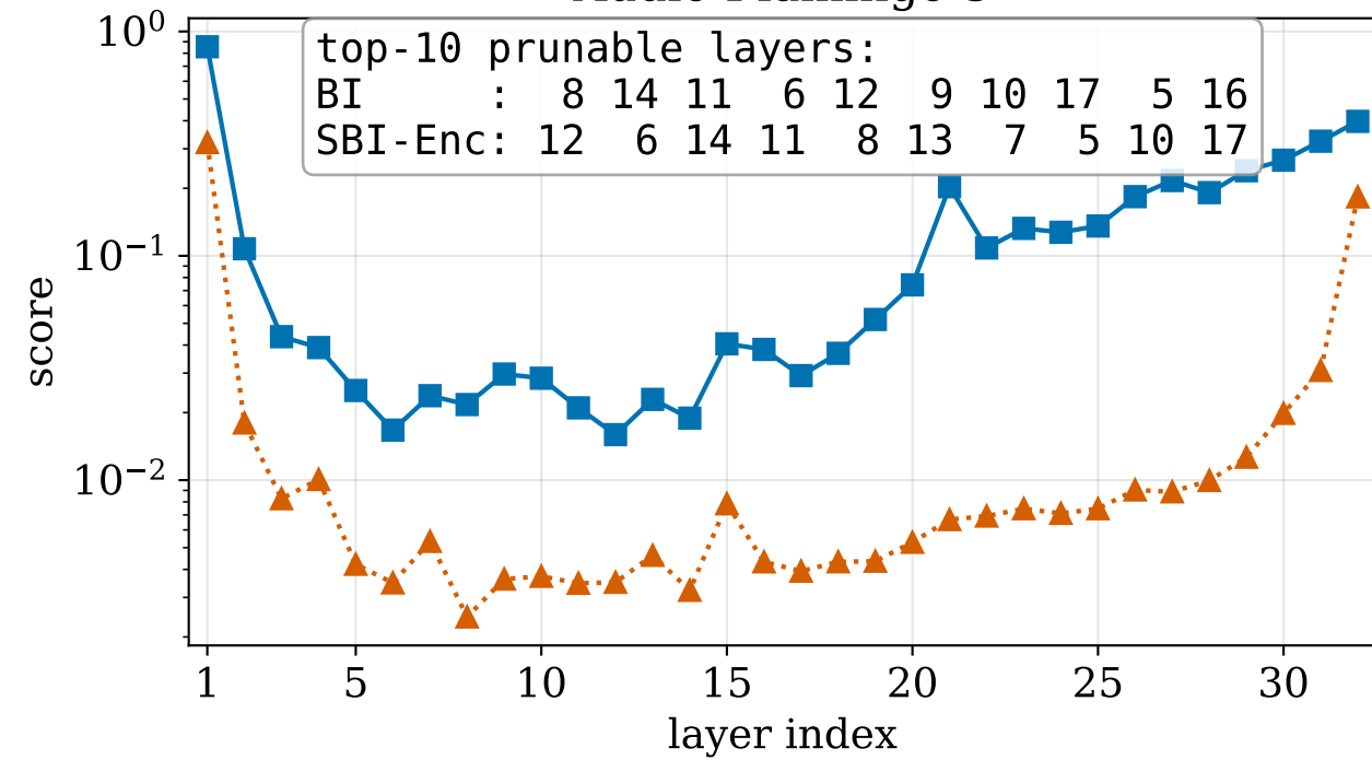
Audio Flamingo 3
