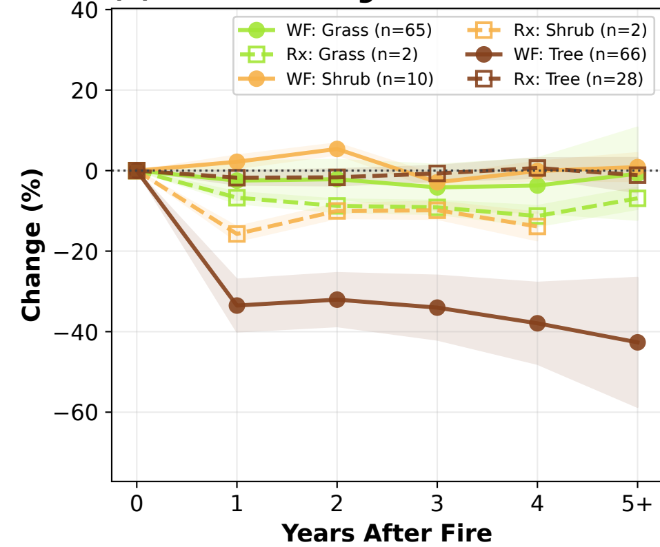
(F) California: Vegetation
