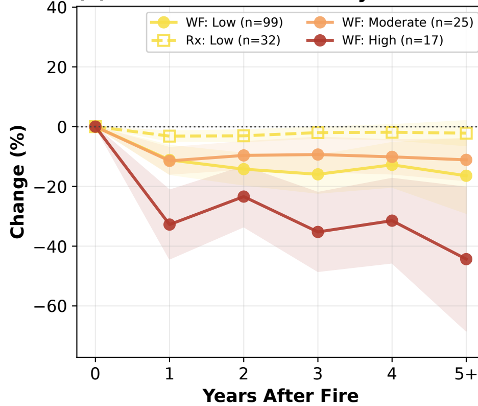
(E) California: Fire Severity
