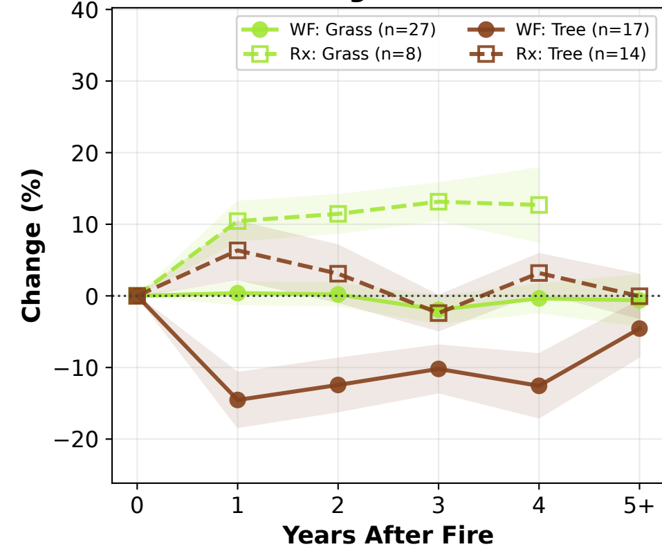
(C) Colorado: Vegetation
