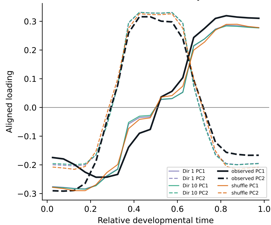
A Observed and null temporal axes
