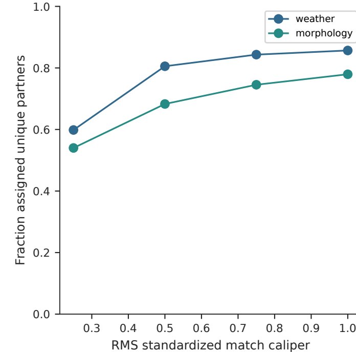
S2F Pairing depends on the caliper
