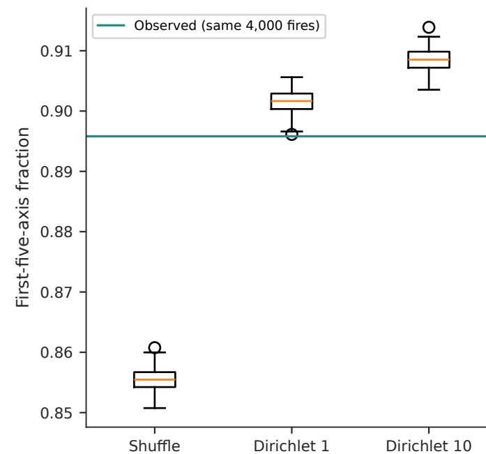
S2B Compression is not uniquely biological
