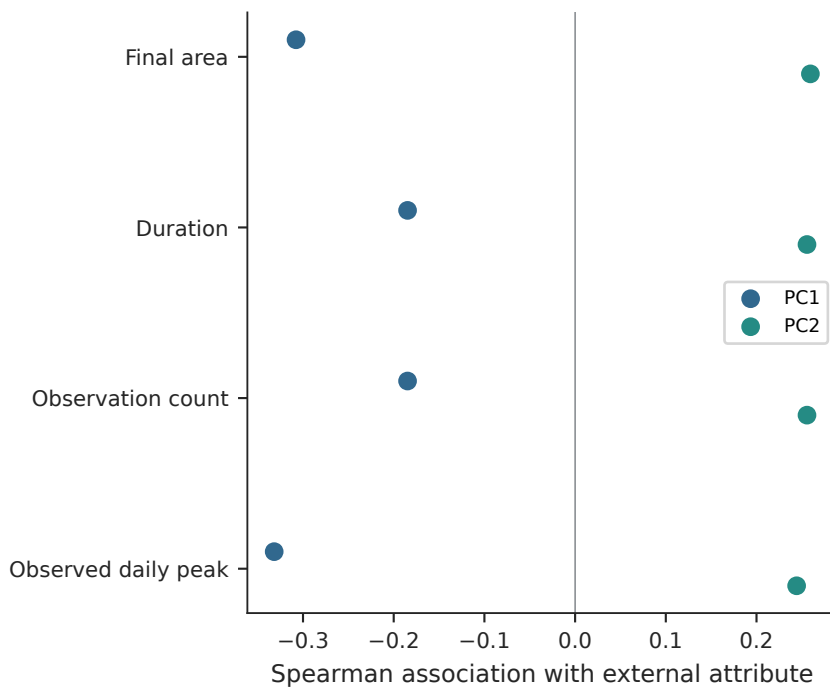
S2D Exclusion does not imply independence
