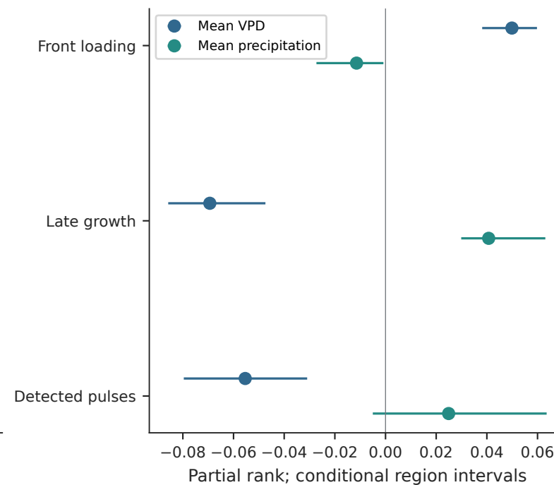
S2E Associations after all coarse controls
