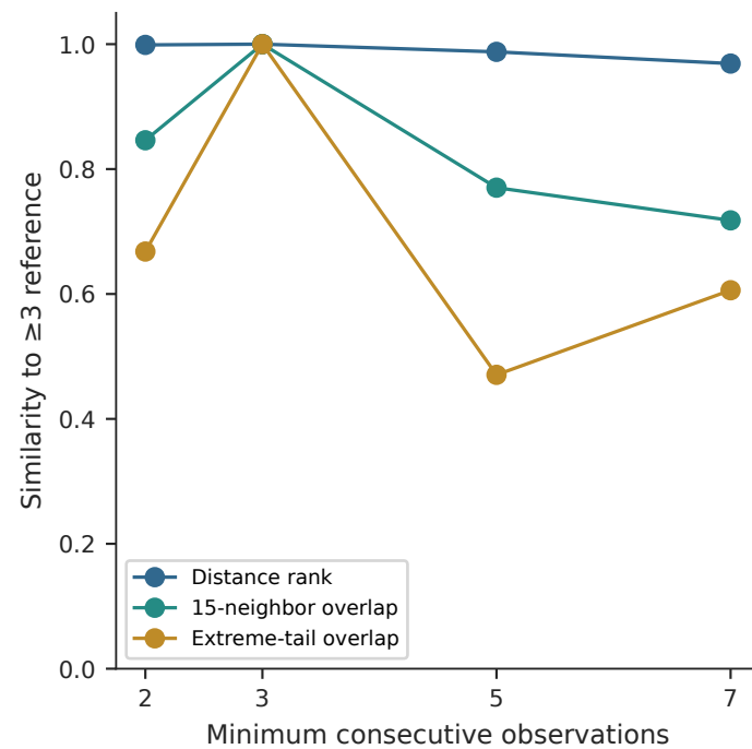
S2D Exclusion does not imply independence
