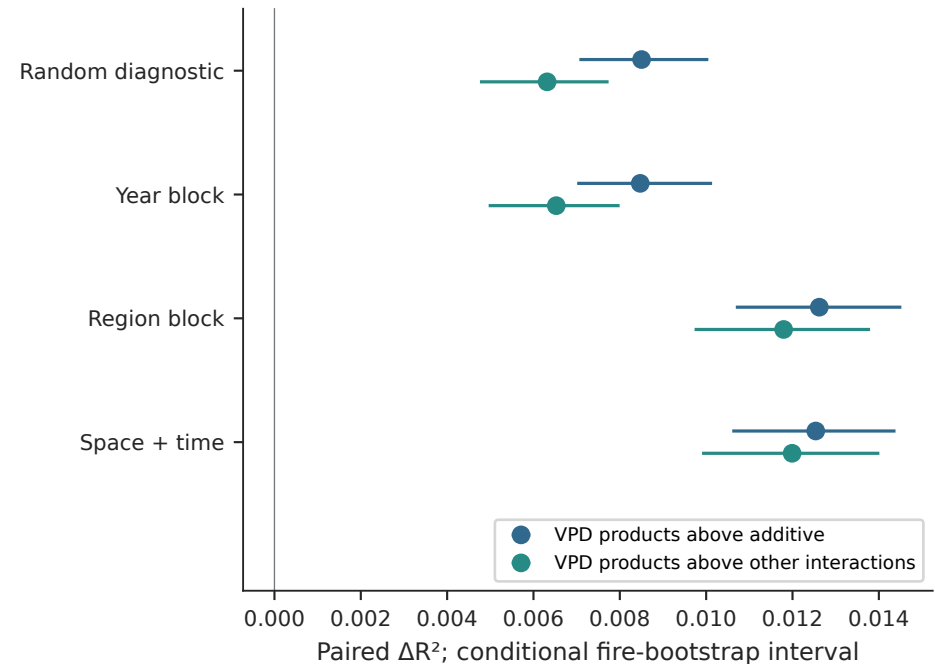
S3D VPD-specific held-out improvement
