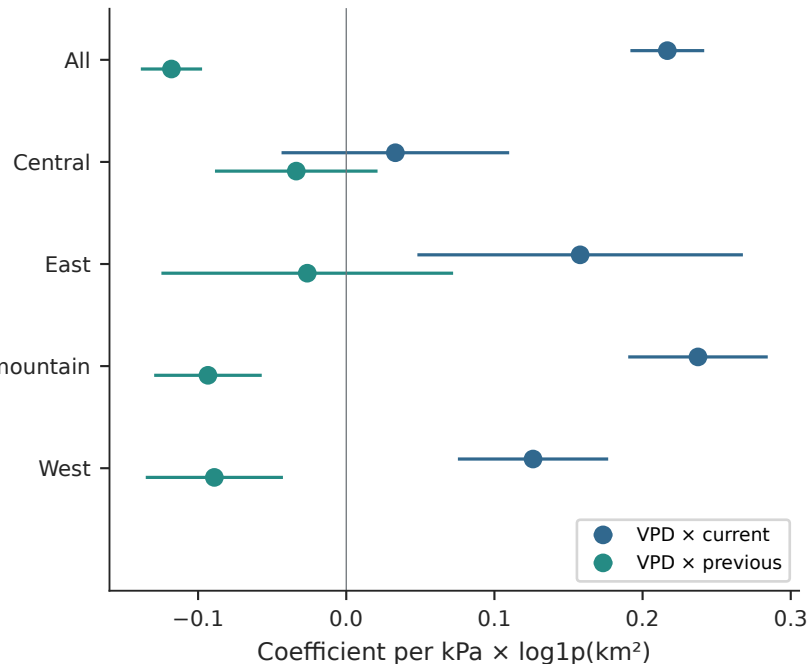
S3C Conditional coefficient heterogeneity
