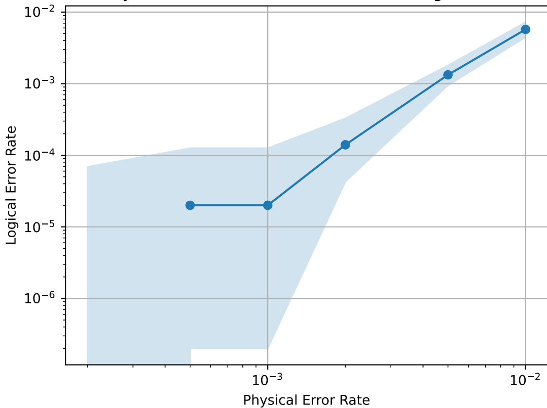
Golay [[23,1,7]] Standalone (Phenomenological Noise)
