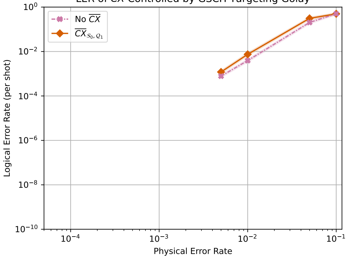
LER of \overline{CX} Controlled by GSCH Targeting Golay
