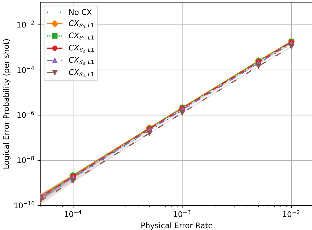
LER of CX Controlled by GSCH Targeting Dodecacode
