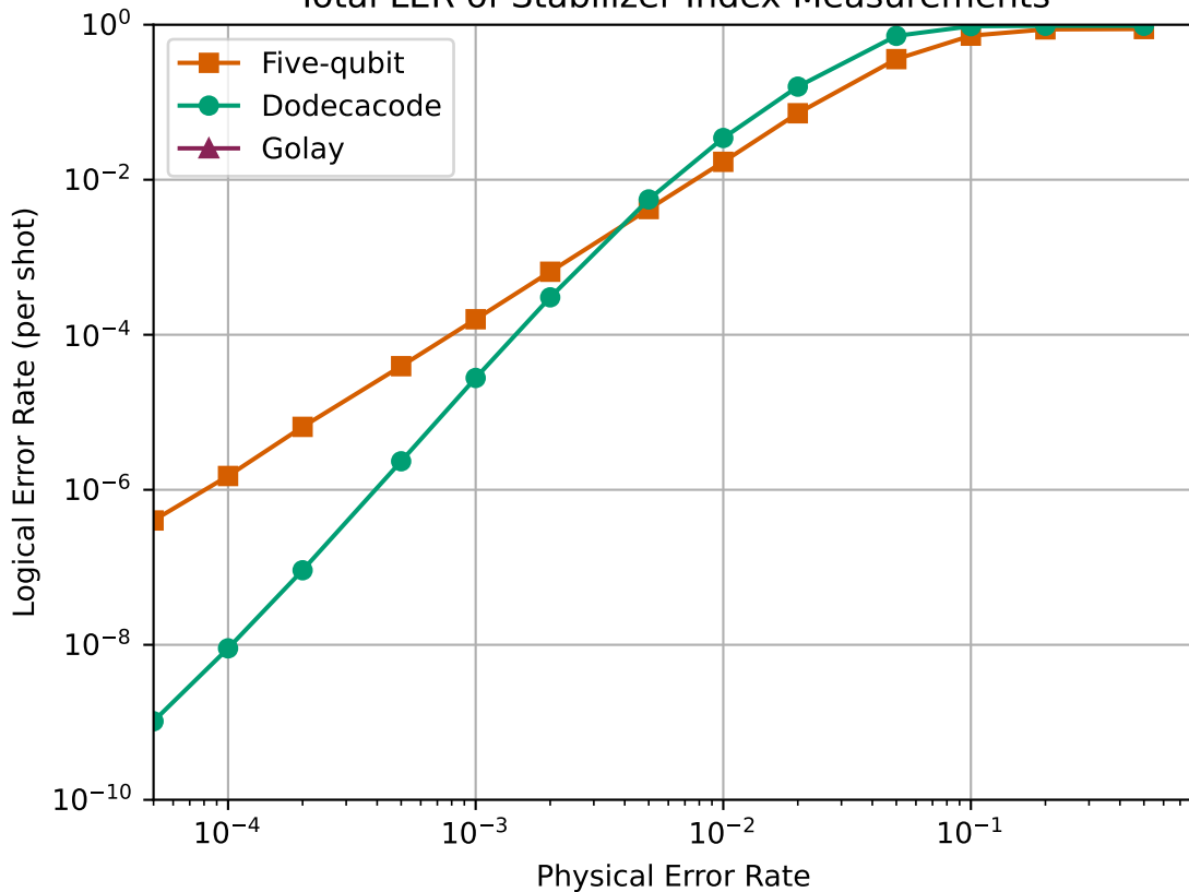
Total LER of Stabilizer Index Measurements
