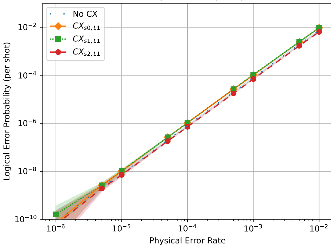
LER of CX Controlled by GSCH Targeting Five Qubit Code
