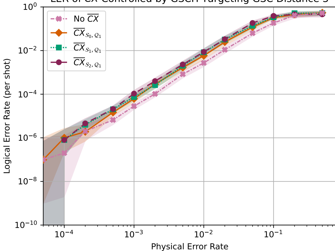
LER of \overline{CX} Controlled by GSCH Targeting GSC Distance 3
