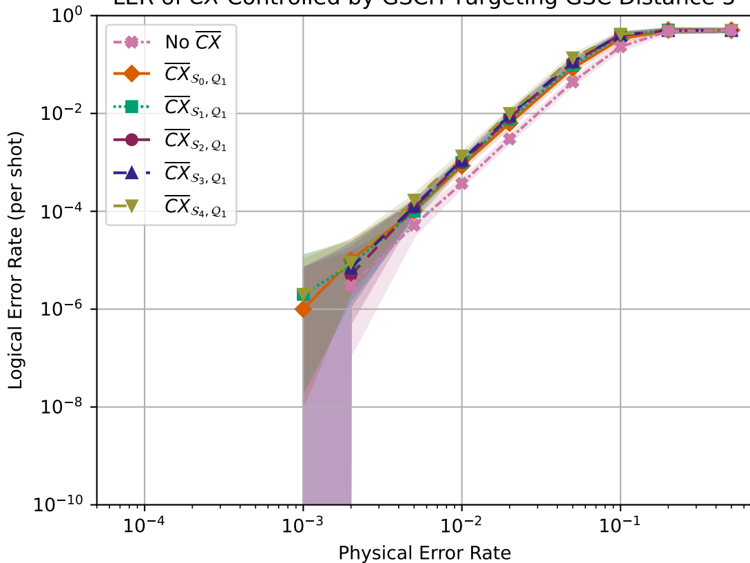
LER of \overline{CX} Controlled by GSCH Targeting GSC Distance 5
