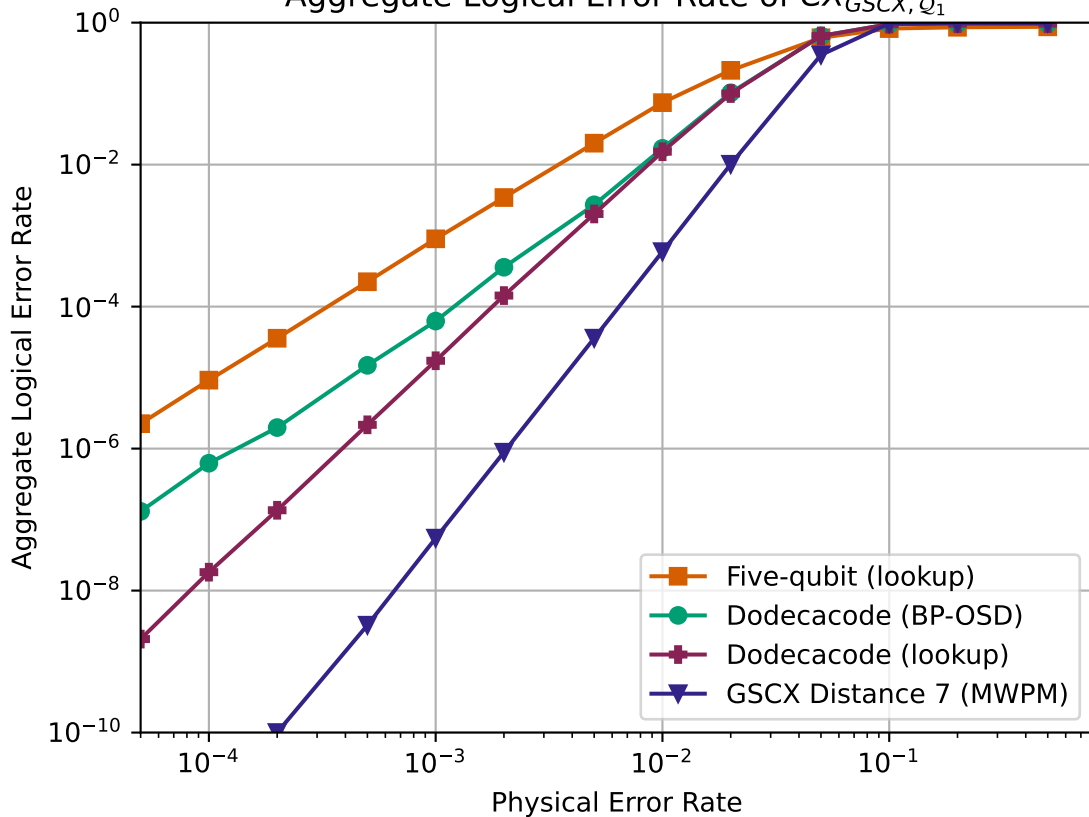
Aggregate Logical Error Rate of \overline{CX}_{GSCX, Q_1}
