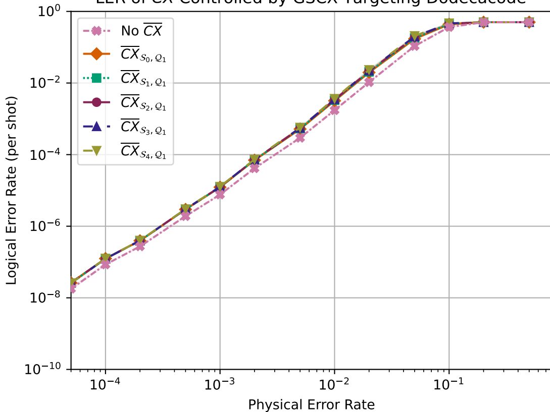
LER of \overline{CX} Controlled by GSCX Targeting Dodecacode
