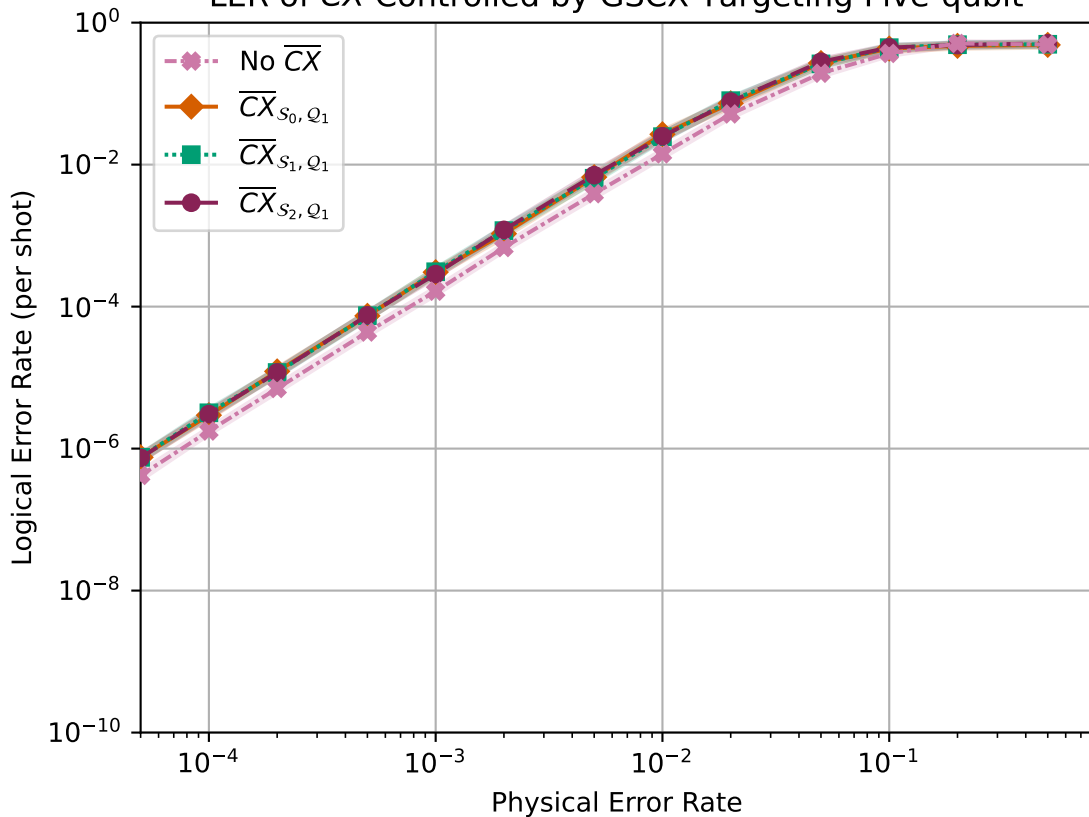
LER of \overline{CX} Controlled by GSCX Targeting Five-qubit
