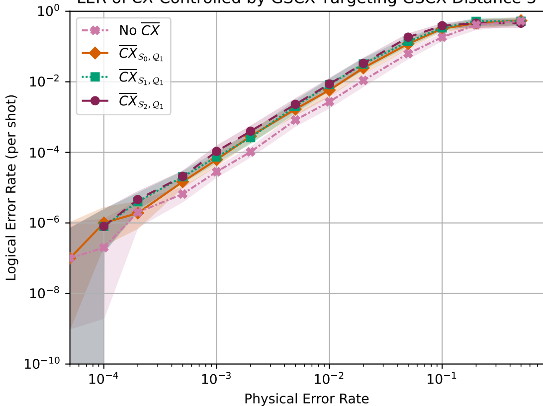
LER of \overline{CX} Controlled by GSCX Targeting GSCX Distance 3
