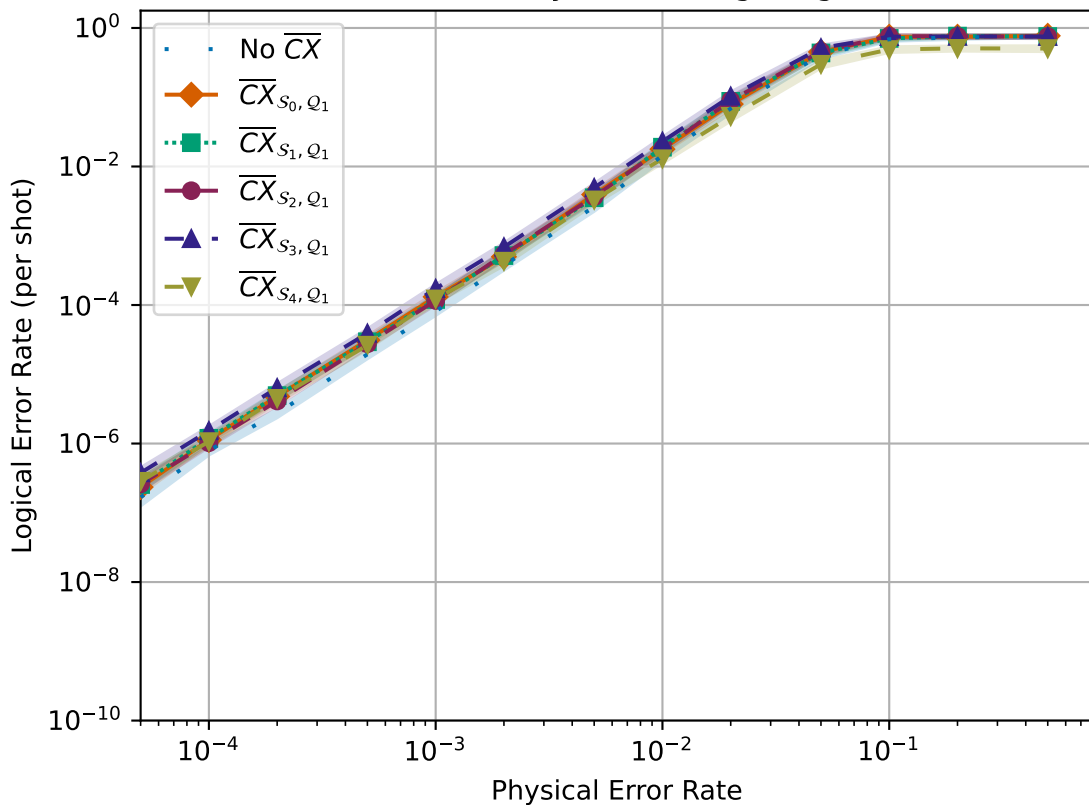
LER of \overline{CX} Controlled by GSCH Targeting Dodecacode
