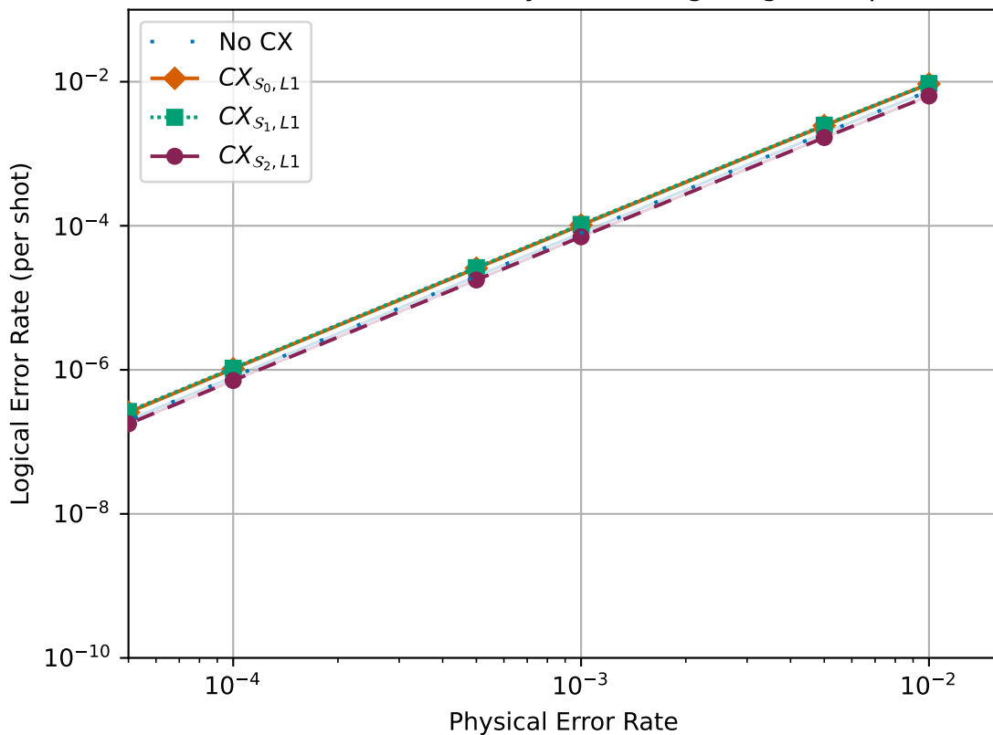
LER of CX Controlled by GSCH Targeting Five-qubit
