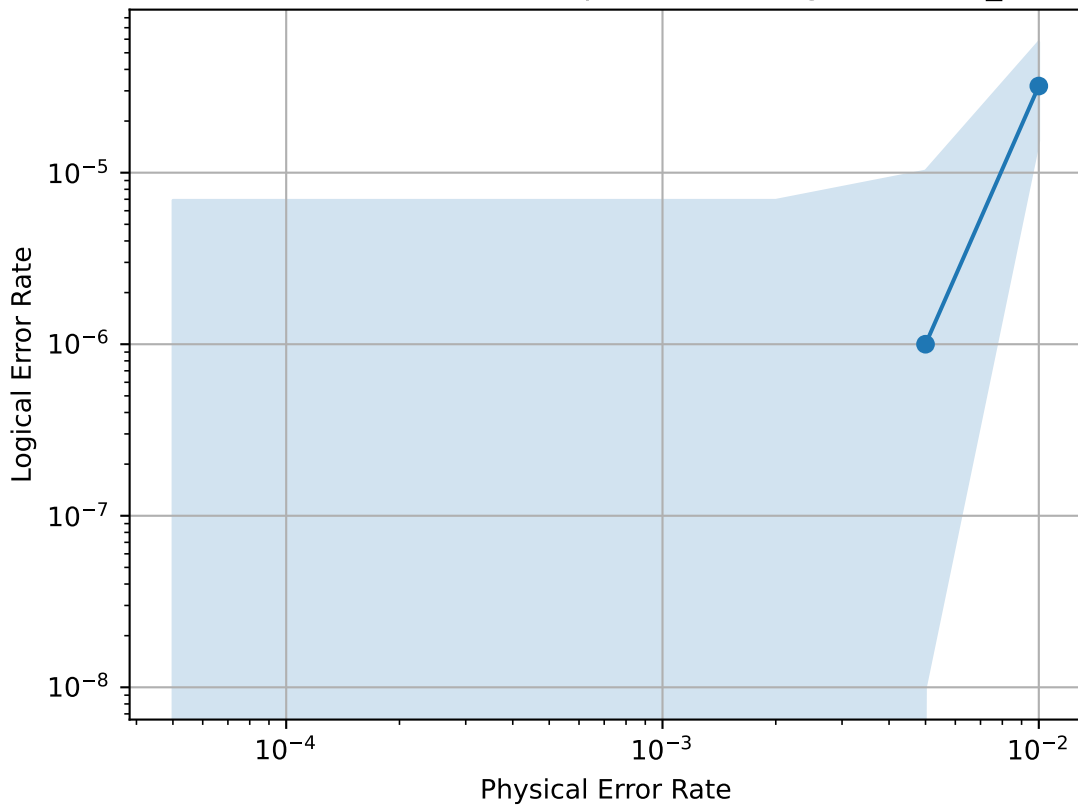
GSC [[49,1,7]] Standalone (phenomenological, exact_mw)
