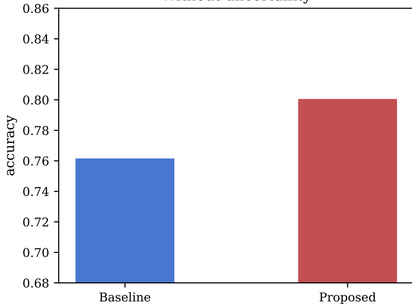
Without uncertainty
