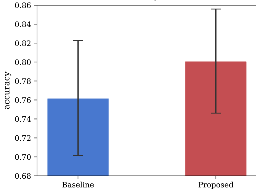
With 95\% CI
