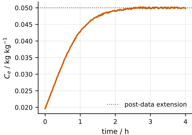
(b) Equivalent equilibrium moisture
