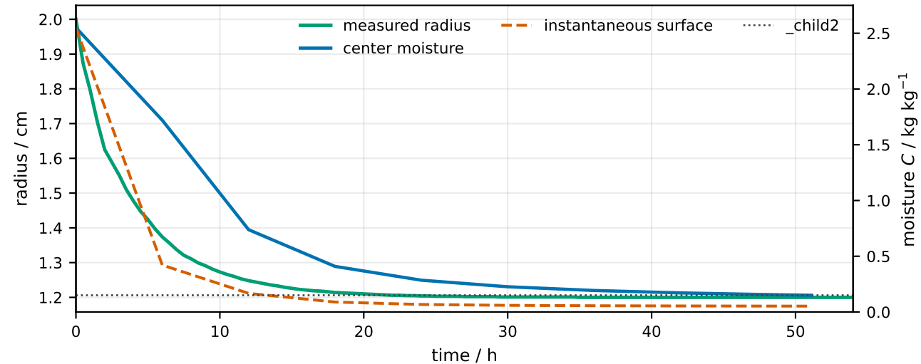
Q4: shrinkage and moisture histories
