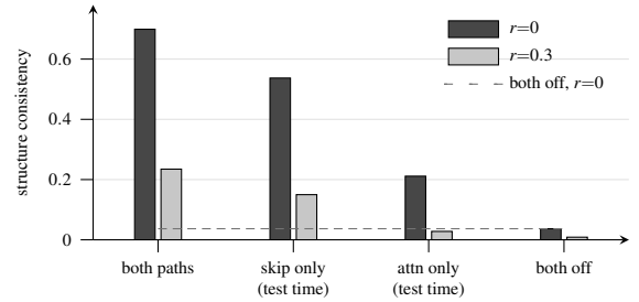
Figure 8: Both injection paths on, then each alone, then neither. The skip residuals carry most of the structure signal; cross-attention alone recovers little of it, and with both off the model falls to the frozen backbone (FID 120.50 against 50.13 with both paths on; skip only 65.12, attention only 67.07). The dashed line is the both-off control at r=0 . Paths are switched off at test time on the trained main model; the separately trained skip-only model is in Table 7. At r=0 the single-path gains over the control roughly add up to the both-paths gain; at r=0.3 the both-paths gain over the control exceeds the sum of the single-path gains.
