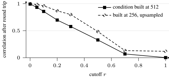
Figure 7: Correlation between the condition fed to the autoencoder and the same condition re-extracted after an encode-decode round trip, 24 images. Above r \approx 0.5 the condition is effectively gone. Building the condition at 256 and upsampling puts the structure at lower absolute frequency and preserves far more, which is why comparisons against older pipelines need the source resolution stated.
