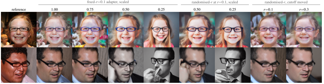
Figure 5: The first two test images under adapter strength and under the cutoff, one seed and caption per row, taken from the runs of Table 2. Lowering the strength of either adapter yields photographs whose pose, framing and colour depart from the reference (the second row turns grayscale at scale 0.25), while moving the cutoff to r=0.3 keeps the reference layout.
