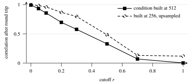
Figure 7: Correlation between the condition fed to the autoencoder and the same condition re-extracted after an encode-decode round trip, 24 images chosen by [AUTHOR-INPUT A37]. Above r\approx 0.5 the condition is effectively gone. Building the condition at 256 and upsampling puts the structure at lower absolute frequency and preserves far more, which is why comparisons against older pipelines need the source resolution stated.
