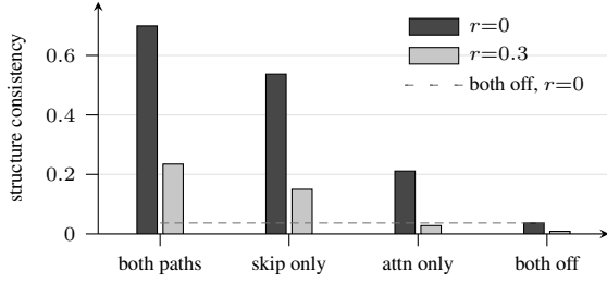
Figure 7: Both injection paths on, then each alone, then neither. The skip residuals carry most of the structure signal; cross-attention alone recovers little of it, and with both off the model falls to the frozen backbone (FID 120.50 against 50.13 with both paths on; skip only 65.12, attention only 67.07). The dashed line is the both-off control at r=0 . At r=0 the single-path gains over the control roughly add up to the both-paths score; at r=0.3 both paths together exceed that sum.
