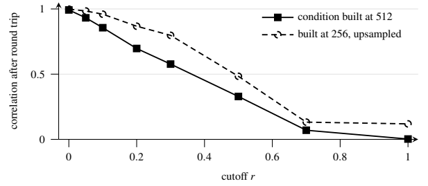
Figure 7: Correlation between the condition fed to the autoencoder and the same condition re-extracted after an encode-decode round trip, 24 images. Above r \approx 0.5 the condition is effectively gone. Building the condition at 256 and upsampling puts the structure at lower absolute frequency and preserves far more, which is why comparisons against older pipelines need the source resolution stated.
